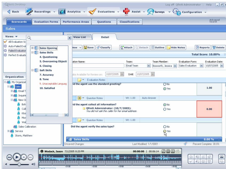
Figure 2: Qfiniti Enterprise User Interface
