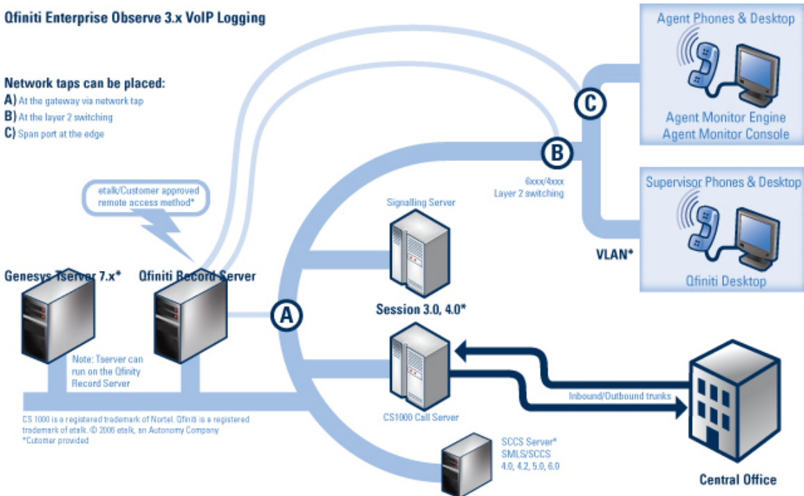
Figure 1: Nortel LAN Tapping Positions
